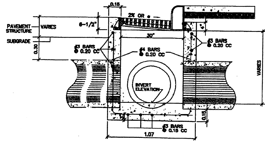
SECTION J-J
