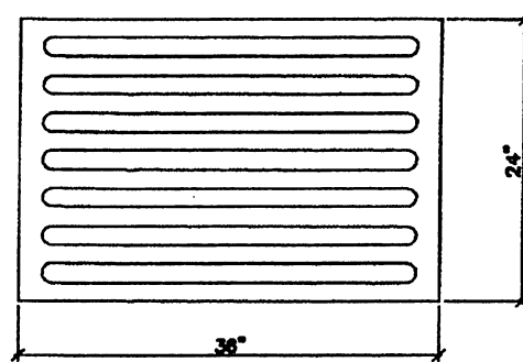
ALTERNATE GRATE
