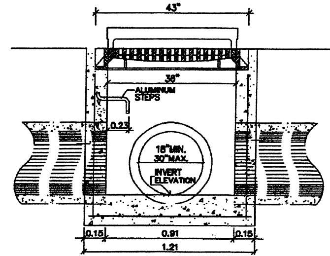
SECTION I-I
