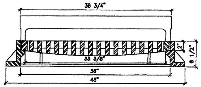
SECTION I-I
