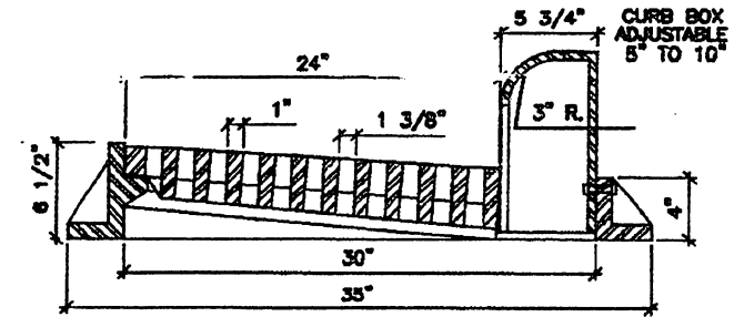
SECTION K-K
