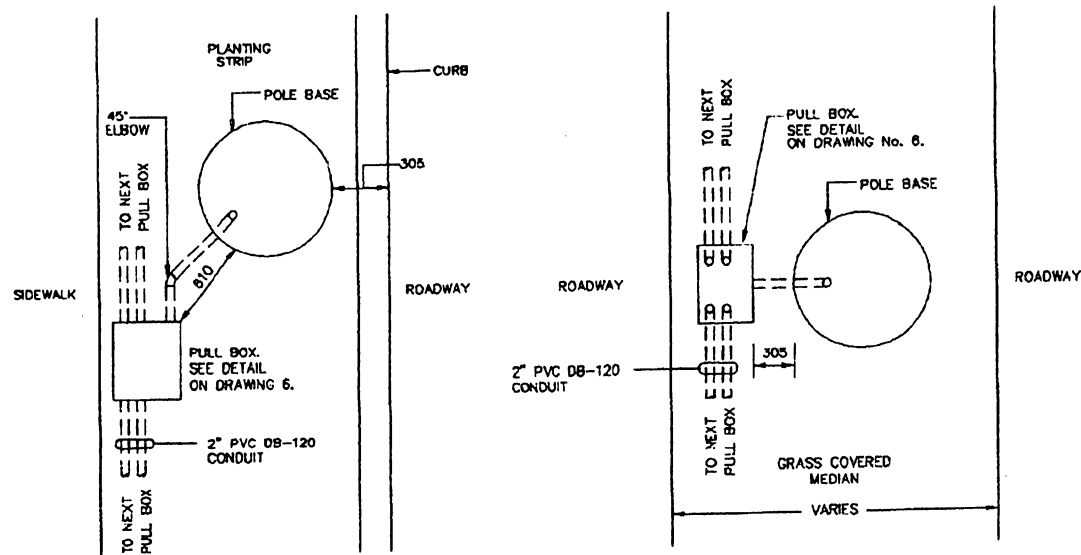
MEDIAN INSTALLATION NOT TO SCALE
