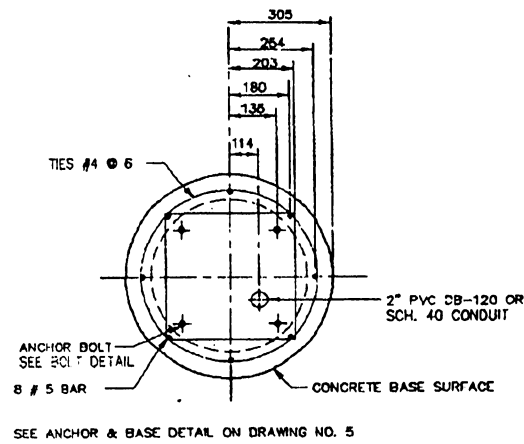
CONC. BASE TOP VIEW (TRANSFORMER OR SHOE BASE) NOT TO SCALE
