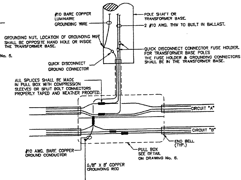
LIGHTING POLE CONNECTION DETAIL NOT TO SCALE
