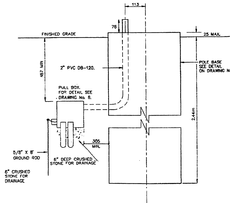
DETAIL OF PULL BOXES FOR LIGHTING CIRCUITS NOT TO SCALE
