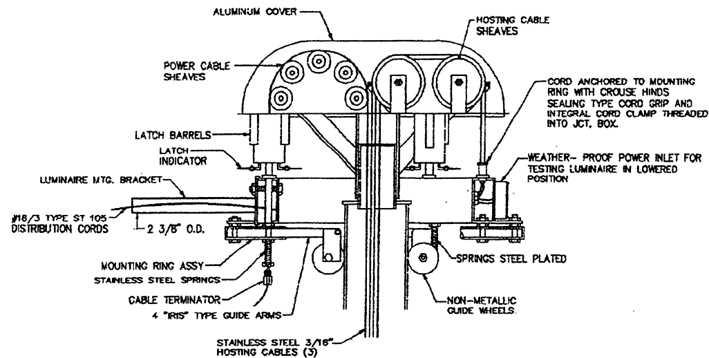
HEAD FRAME AND MOUNTING RING ASSEMBLY SCALE: N.T.S.
