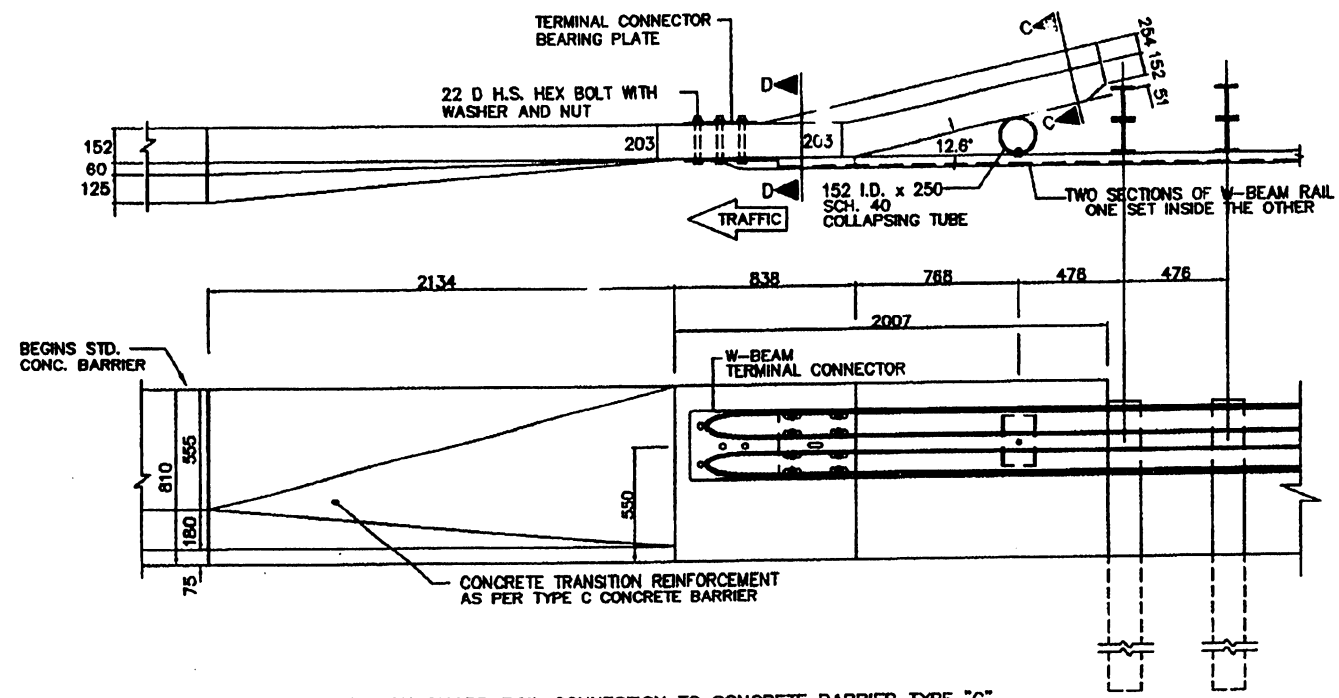
TRANSITION GUARD RAIL CONNECTION TO CONCRETE BARRIER TYPE "C" FOR POST SPACING TRANSITION SEE GUARD RAIL TRANSITION TO CONCRETE BRIDGE PARAPET.
