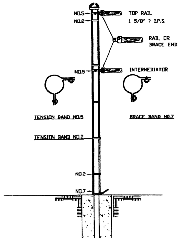
CORNER POST DETAILS NOT TO SCALE
