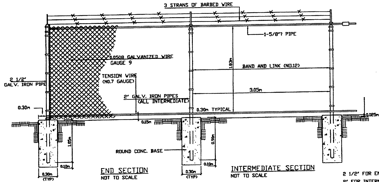
TYPICAL INSTALLATION
