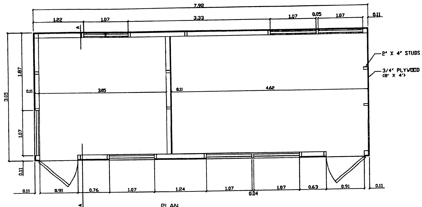
PLAN SCALE 1/24
