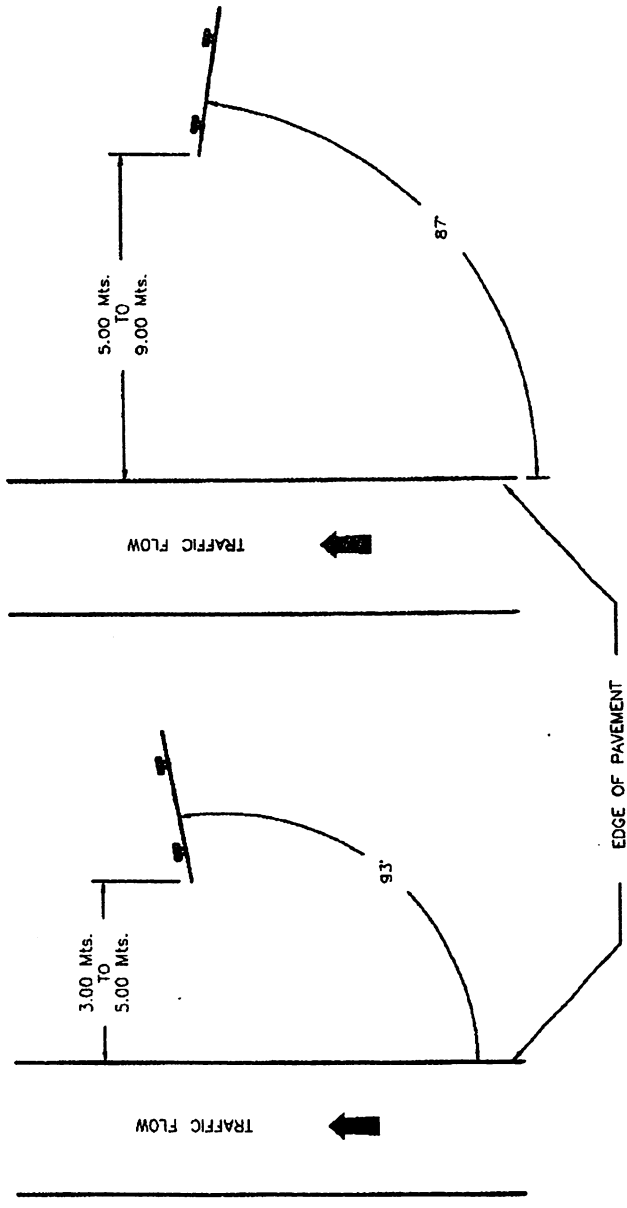
ORIENTATION OF SIGNS
