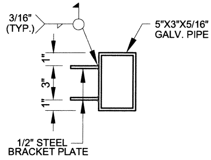
SECTION "D-D" NOT TO SCALE
