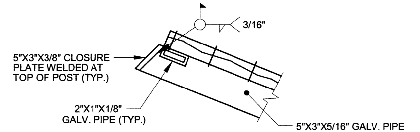
DETAIL "C" NOT TO SCALE
