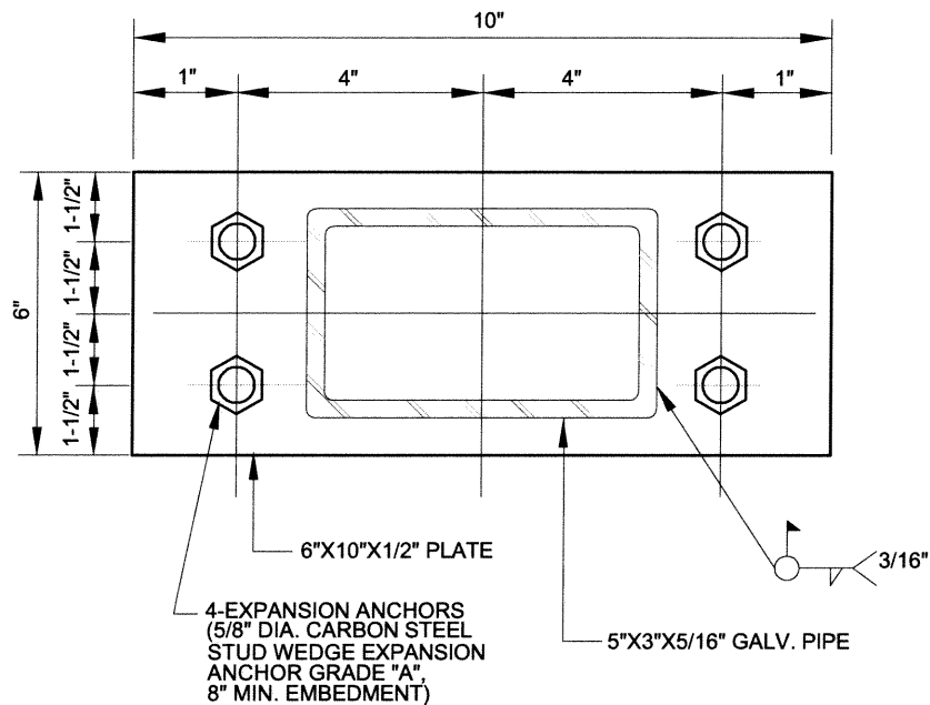
SECTION "B-B" NOT TO SCALE
