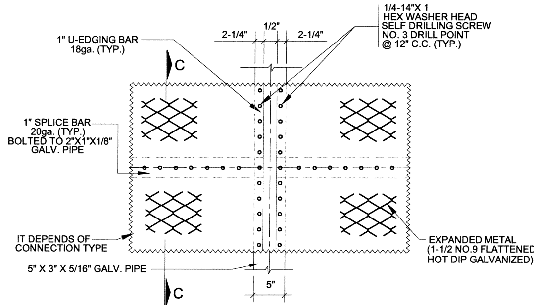
TYPICAL DETAIL OF EXPANDED METAL POST CONNECTION NOT TO SCALE
