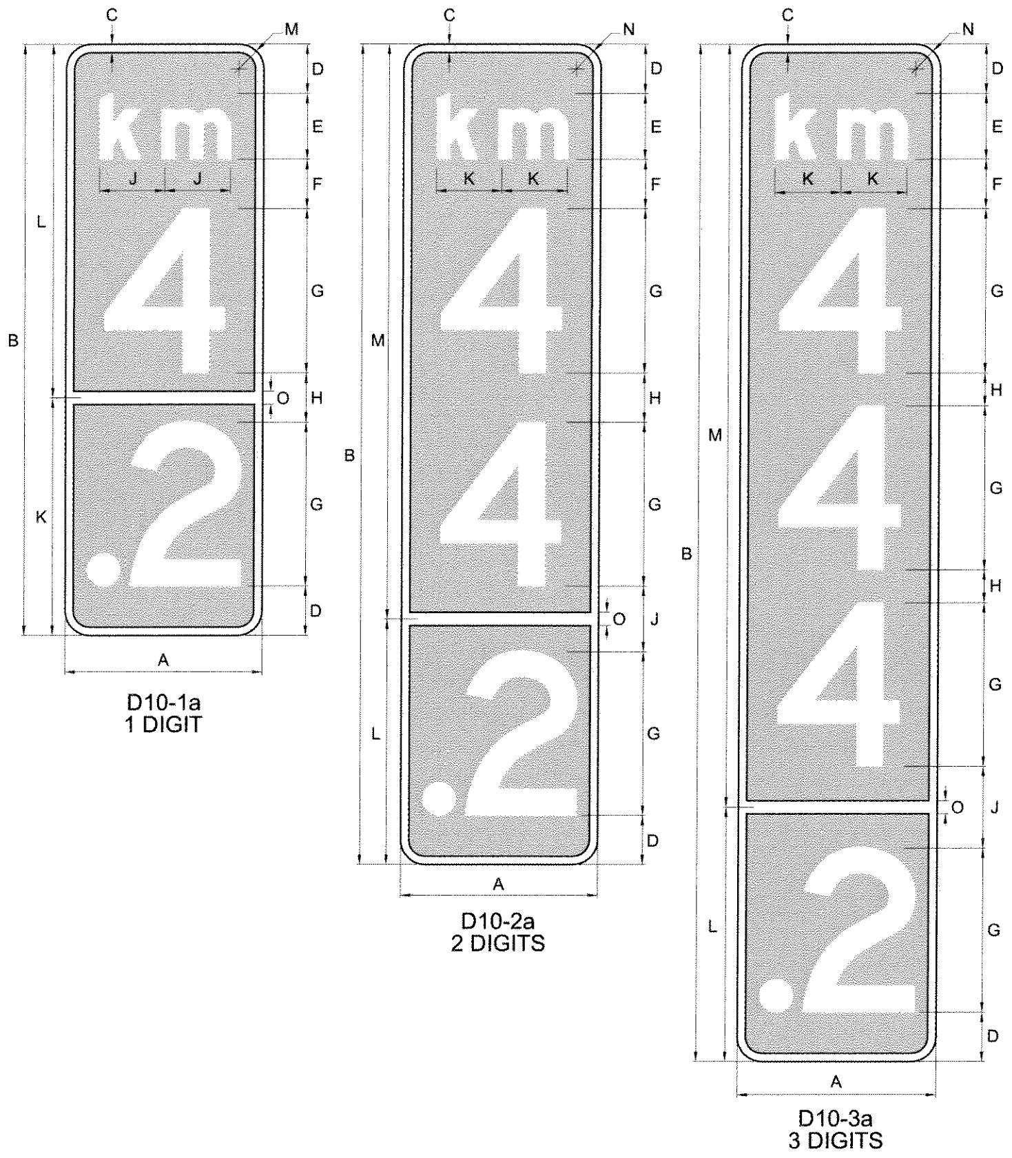
KILOMETER AND HECTOMETER PANEL NOT TO SCALE
