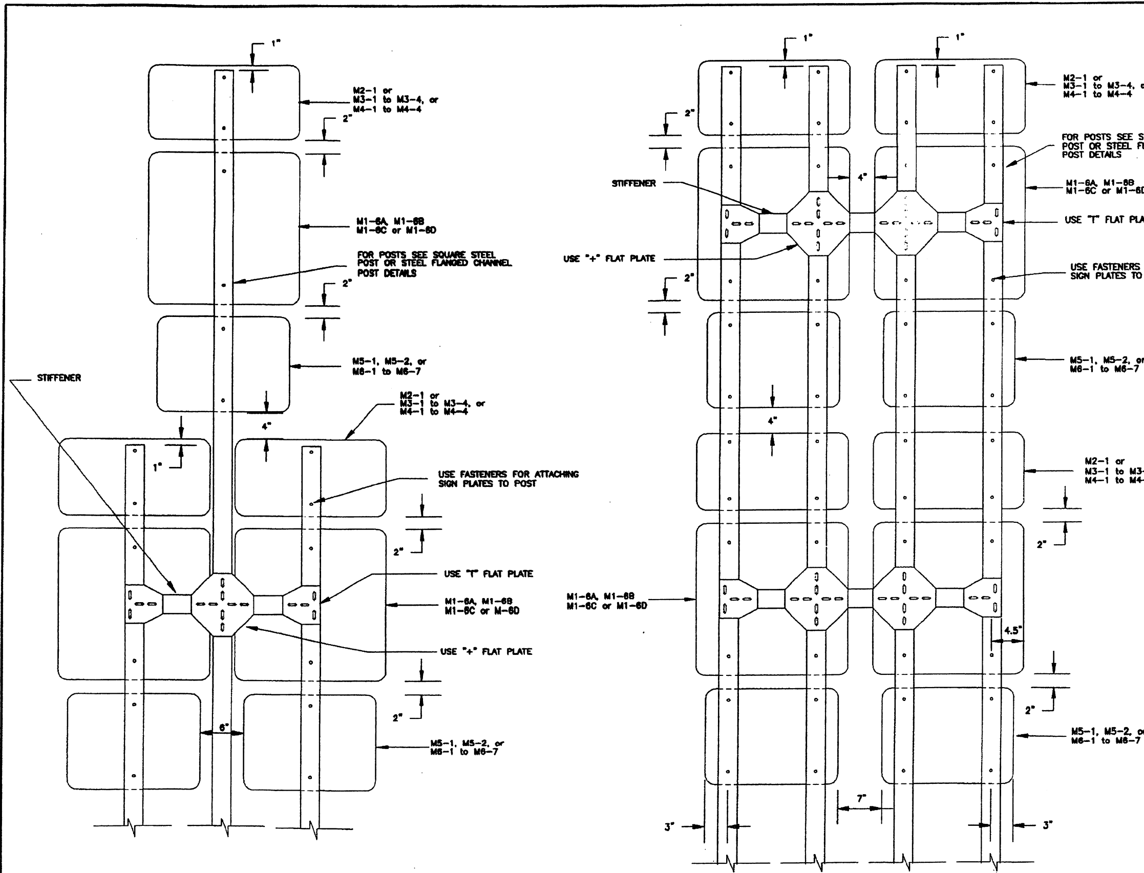
TYPICAL ROUTE MARKER ASSEMBLY FOR THREE 24"x24" ROUTE MARKERS WITH OR WITHOUT AUXILIARY PLATES
