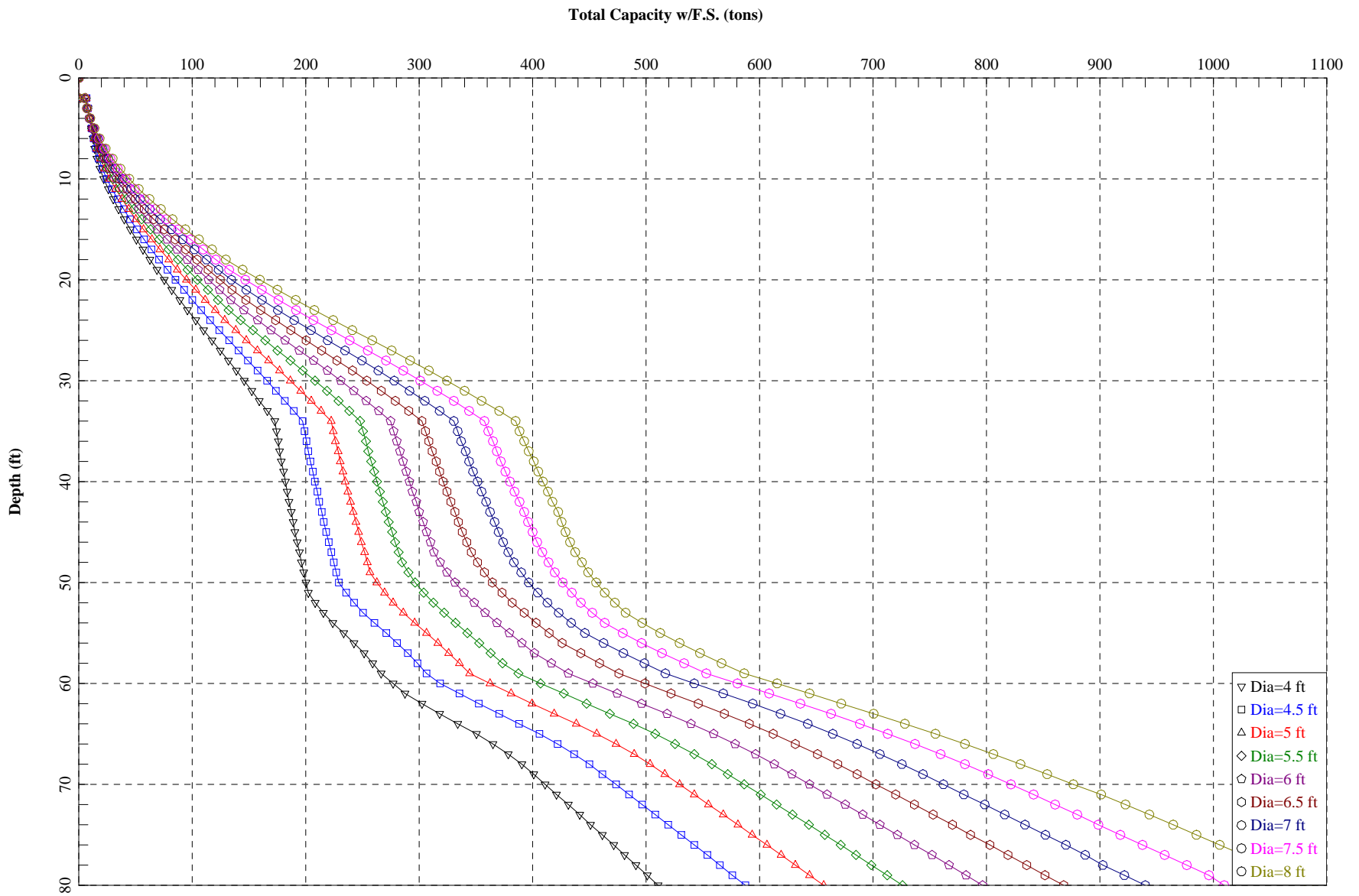
Depth vs. Allowable Compressive Axial Load - Drilled Shaft in Boring no. 1
