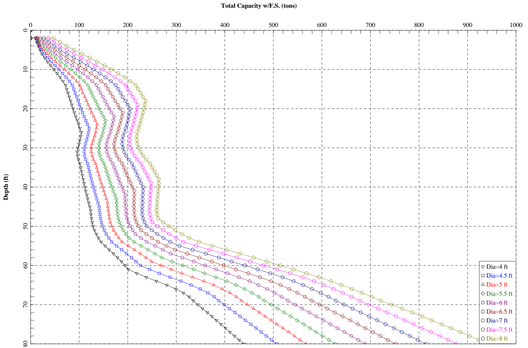
Depth vs. Allowable Compressive Axial Load - Drilled Shaft in Boring no. 5
