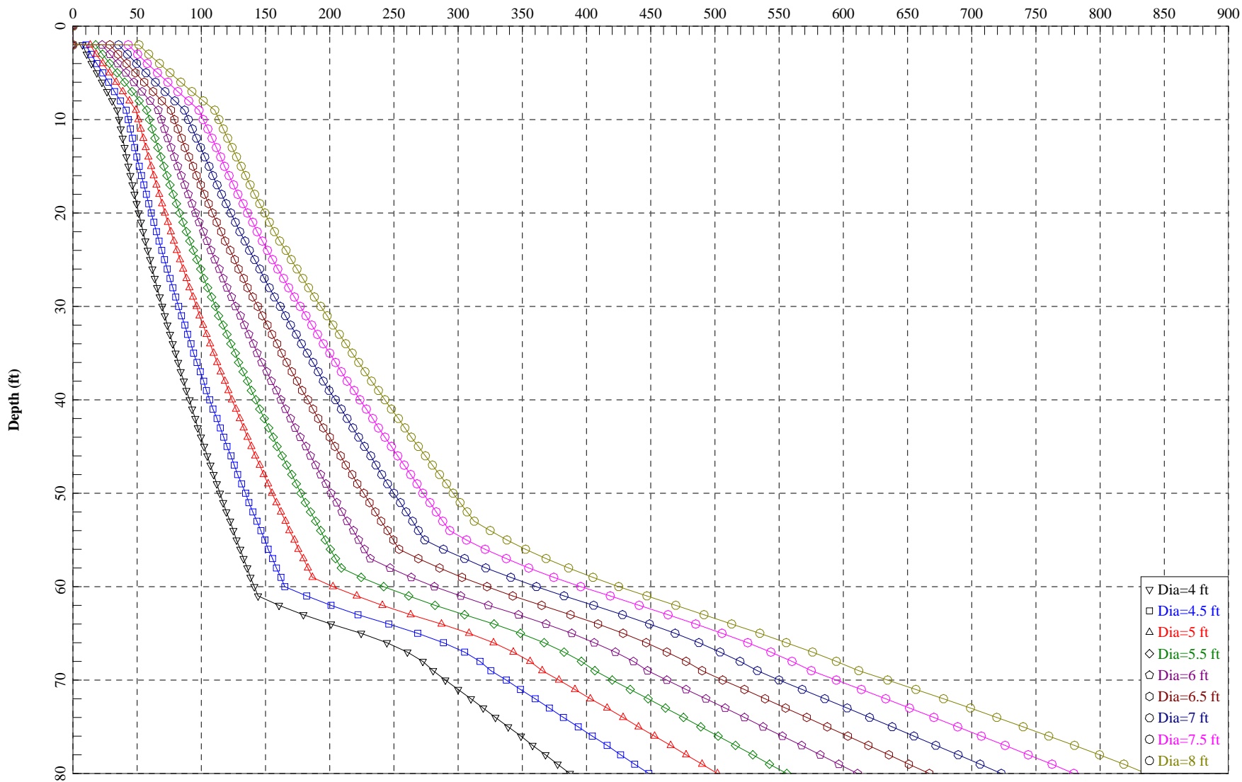
Depth vs. Allowable Compressive Axial Load - Drilled Shaft in Boring no. 4
