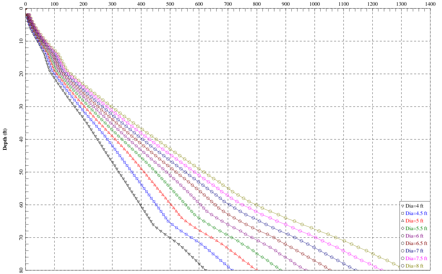
Depth vs. Allowable Compressive Axial Load - Drilled Shaft in Boring no. 3
