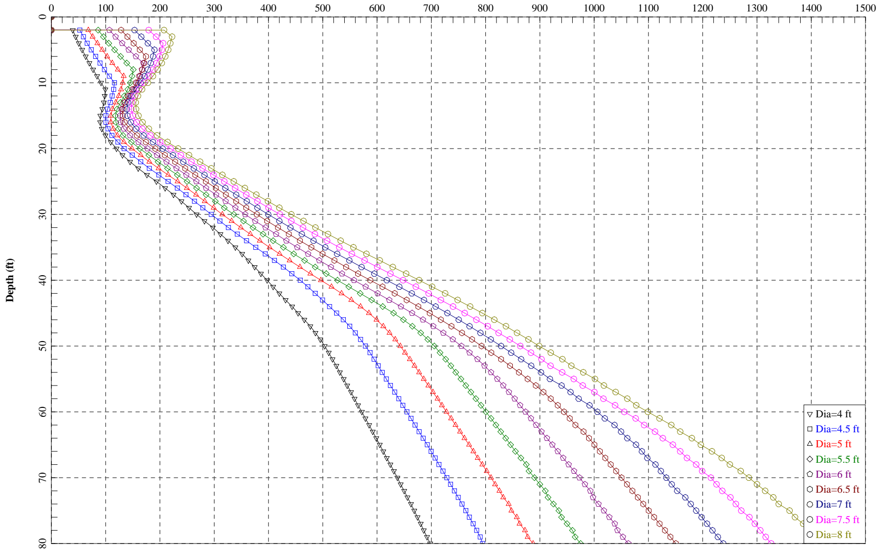
Depth vs. Allowable Compressive Axial Load - Drilled Shaft in Boring no. 6
