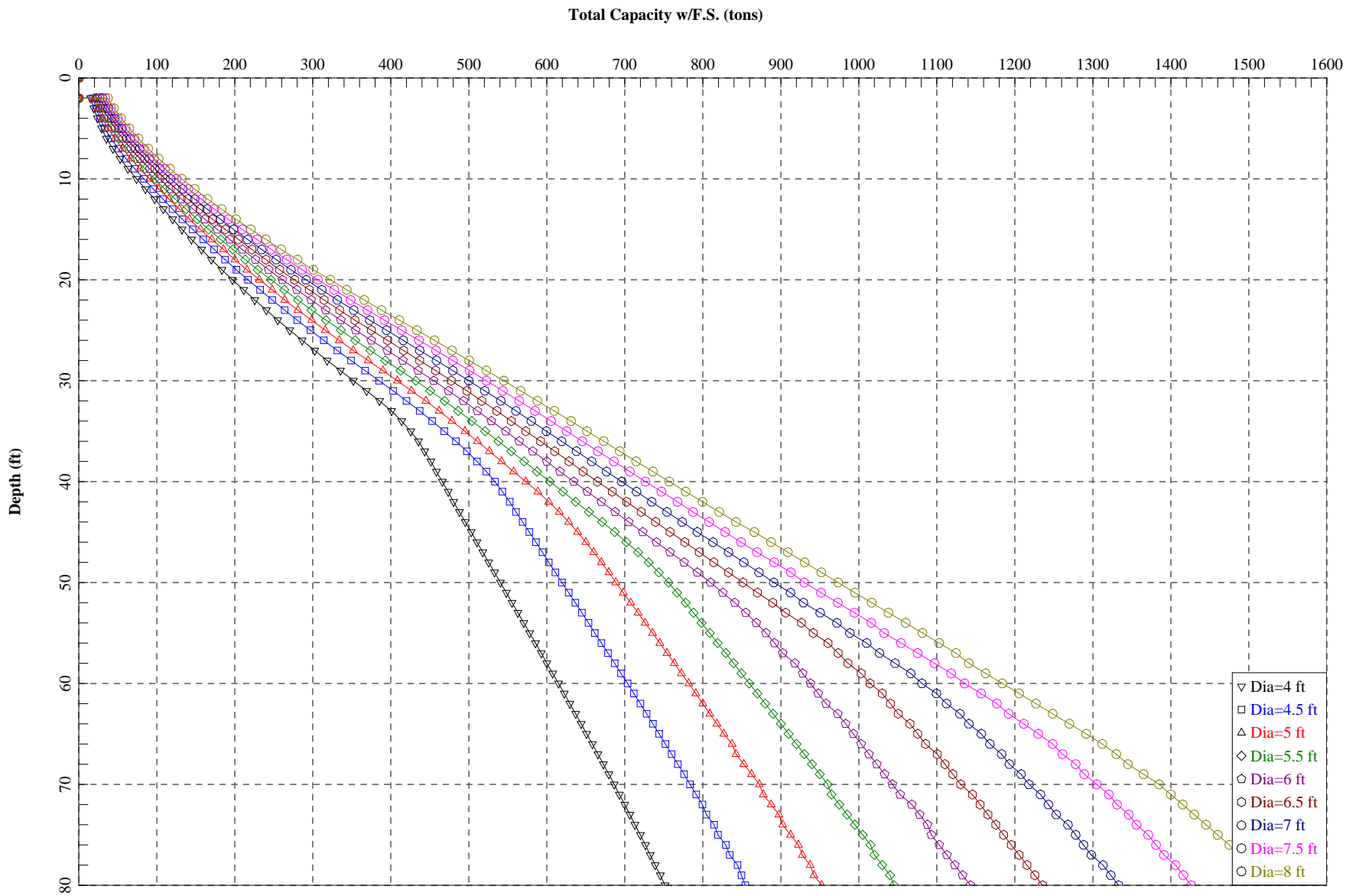
Depth vs. Allowable Compressive Axial Load - Drilled Shaft in Boring no. 2
